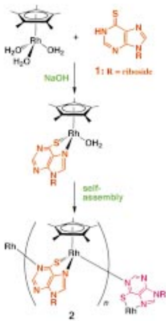
Scheme 1. Expected self-assembling process to form cyclic oligomers.
